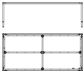
C 87000 Tavolo rettangolare in alluminio, 9 doghe Rectangular table in aluminum, 9 slats cm 240 x 110 x h 73 in 94 1/2 x 43 3/8 x h 28 3/4
