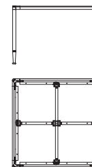
C 87002 Tavolo quadrato in alluminio, 4 doghe Rectangular table in aluminum, 4 slats cm 110 x 110 x h 73 in 43 3/8 x 43 3/8 x h 28 3/4
